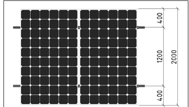
Portrait panel orientation 300W
