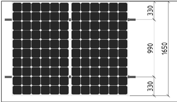
Portrait panel orientation 250W
